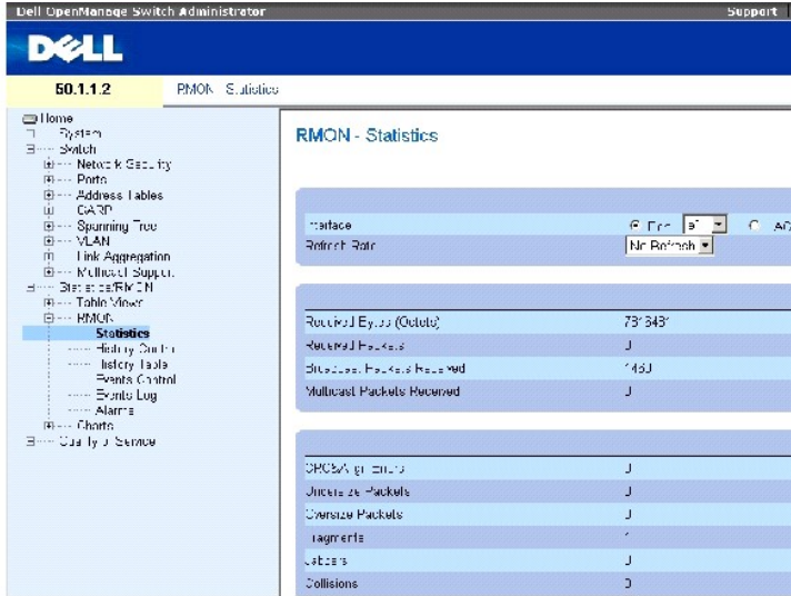
Figura 8-7. RMON Statistics
